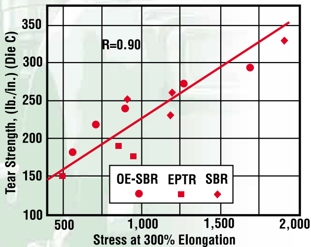
Plot of ASTM Die C Tear Strength as a Function of Stress at 300% Elongation
